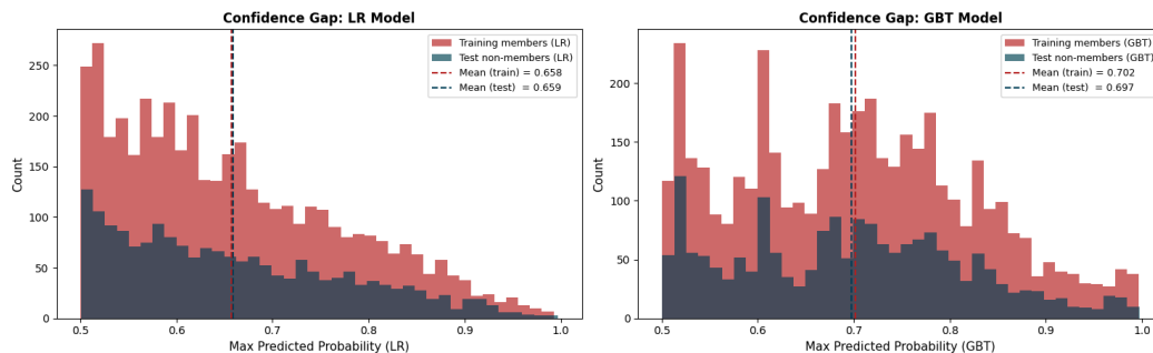
Confidence Gap Histograms: LR vs. GBT Models
